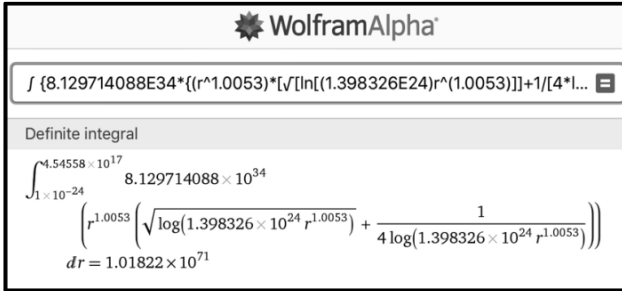
Figure 3. Screenshot of the numerical solution to the integral of eq. (43)
