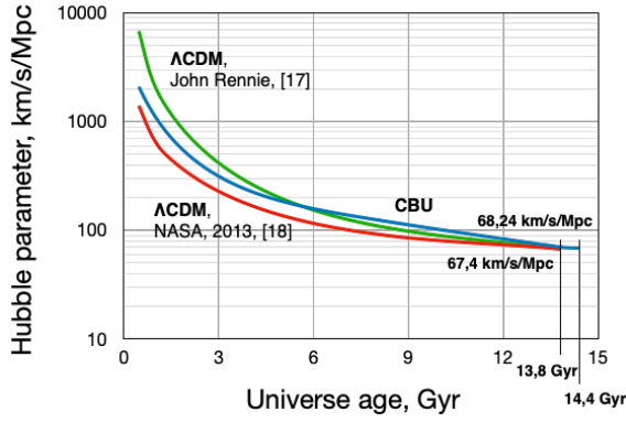
Figure 2. Comparison of the temporal development of the Hubble parameter
