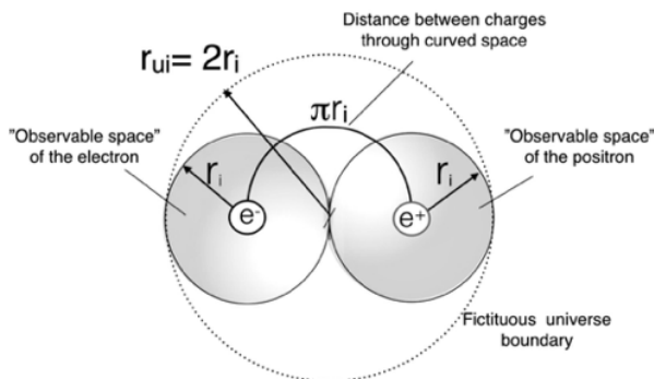
Figure 1. The initial event, according to the hypothesis the universe started from a positron-electron fluctuation
